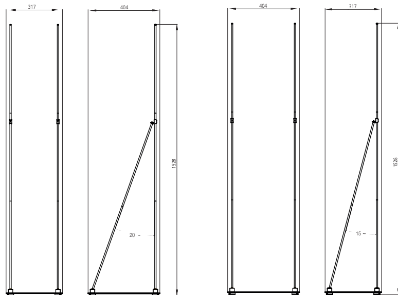
Stand constructed using short side base
